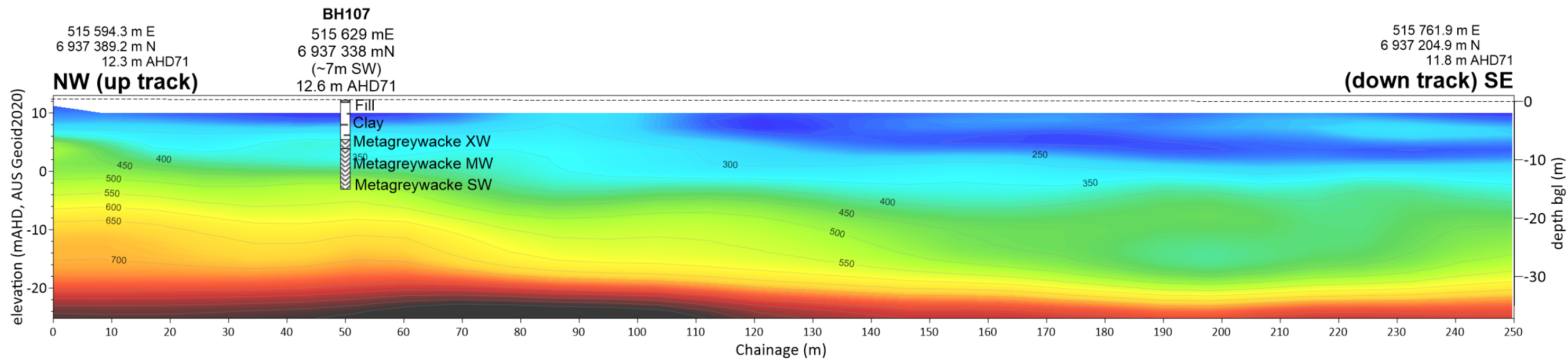
Seismic Line MASW AU-GP 163-2
